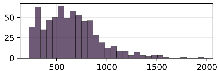
red_edge_1
