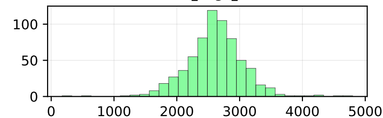
swir_1
