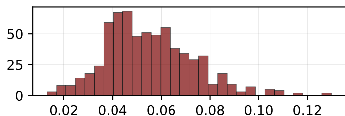
bcmad
