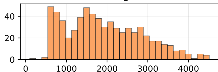
bcmad
