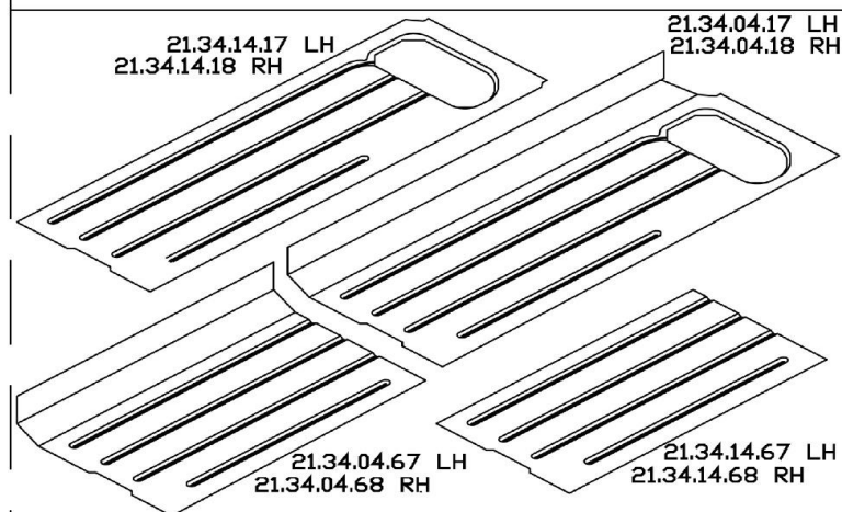
Traveller, Van & Pickup Budget Floor Panels
