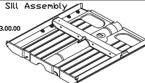
Van/Pickup Floor & Sill Assembly
