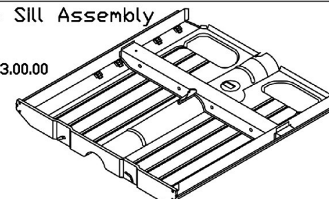
Van/Pickup Floor & Sill Assembly
