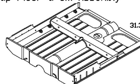
Van/Pickup Floor & Sill Assembly
