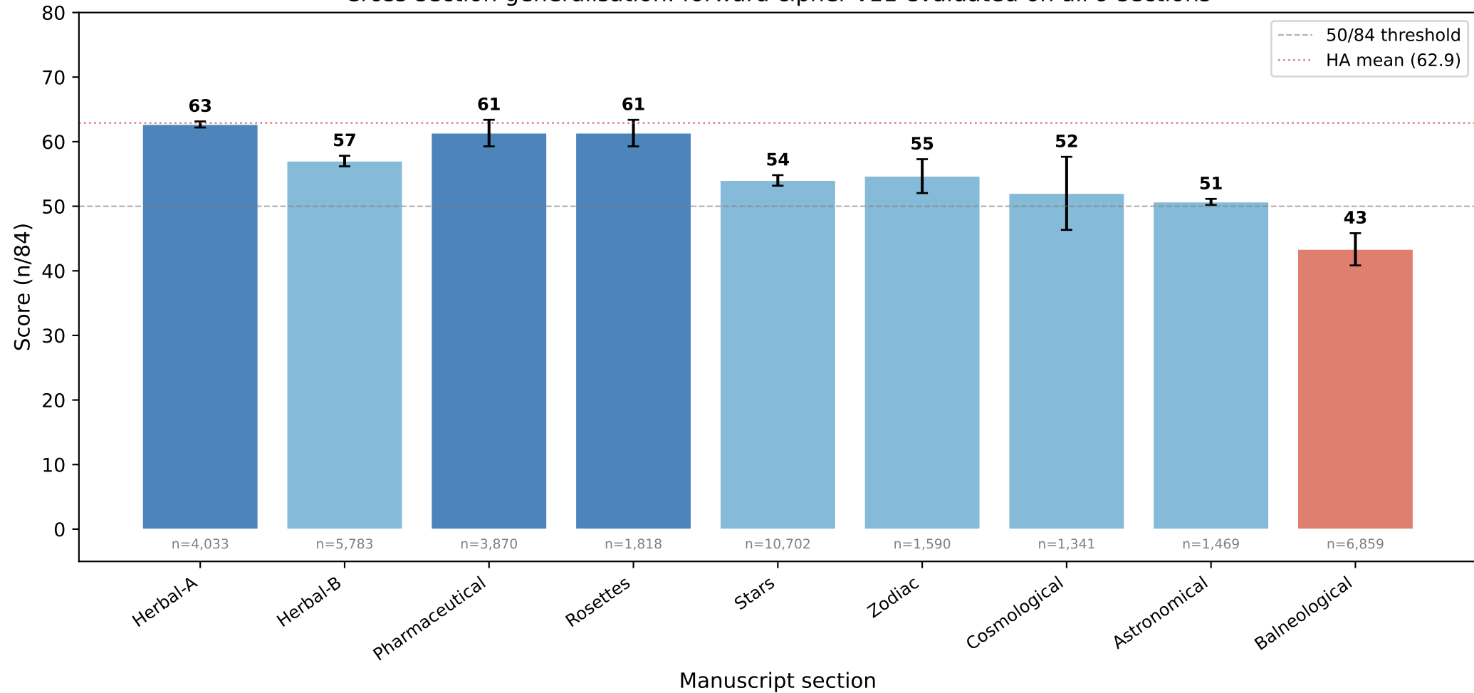
Cross-section generalisation: forward cipher v11 evaluated on all 9 sections
