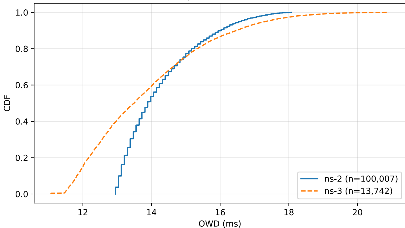
OWD CDF — PQ pktSize=512 KS D=0.3963 p=0 verdict=FAIL ( \alpha=0.05 )
