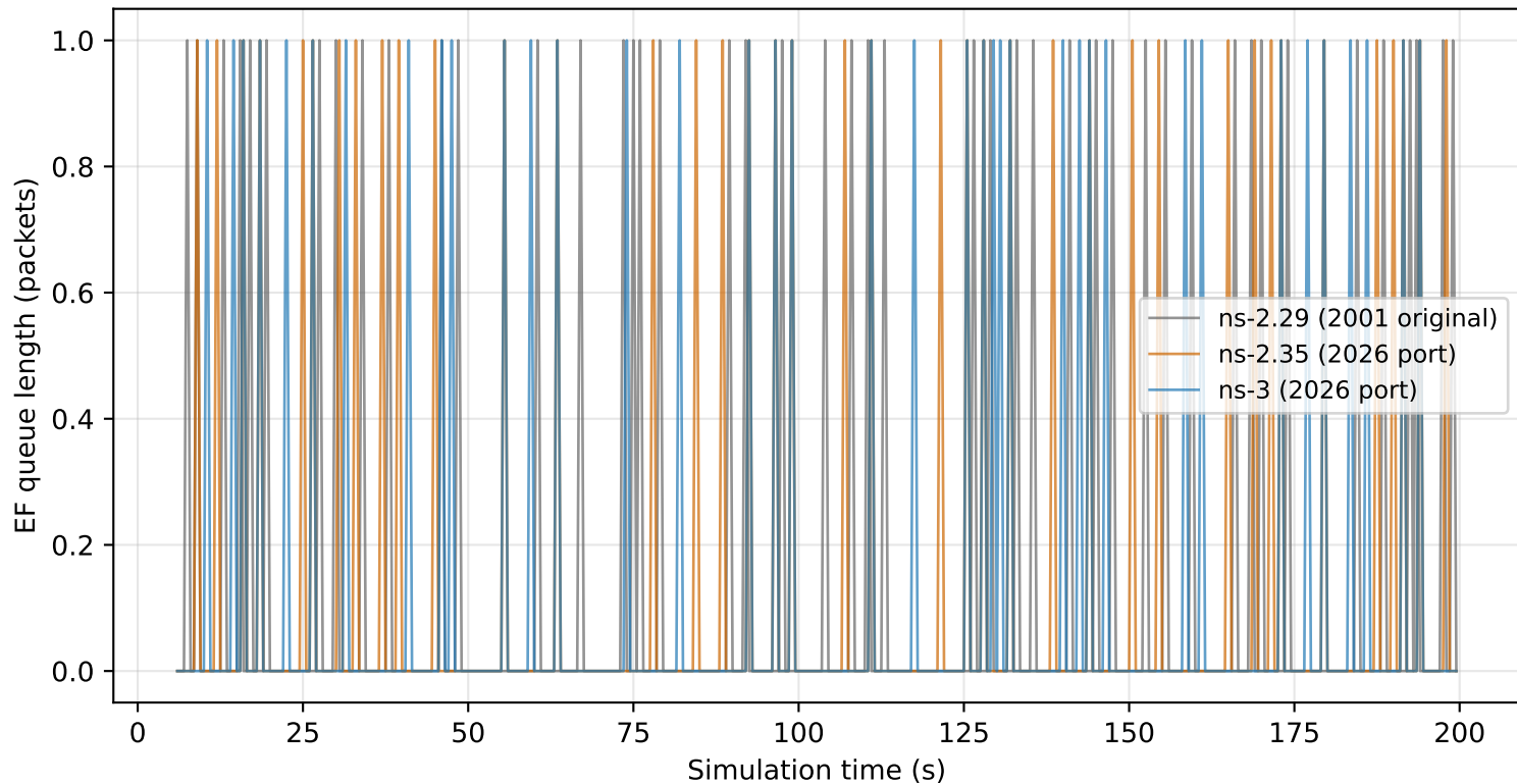
Scenario 1 — EF queue length, 512 B packets
