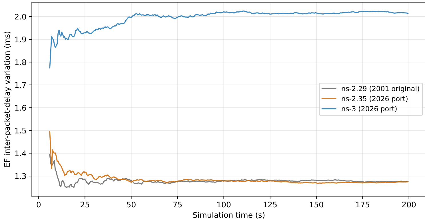
Scenario 1 — EF IPDV at PQ scheduler, 512 B packets
