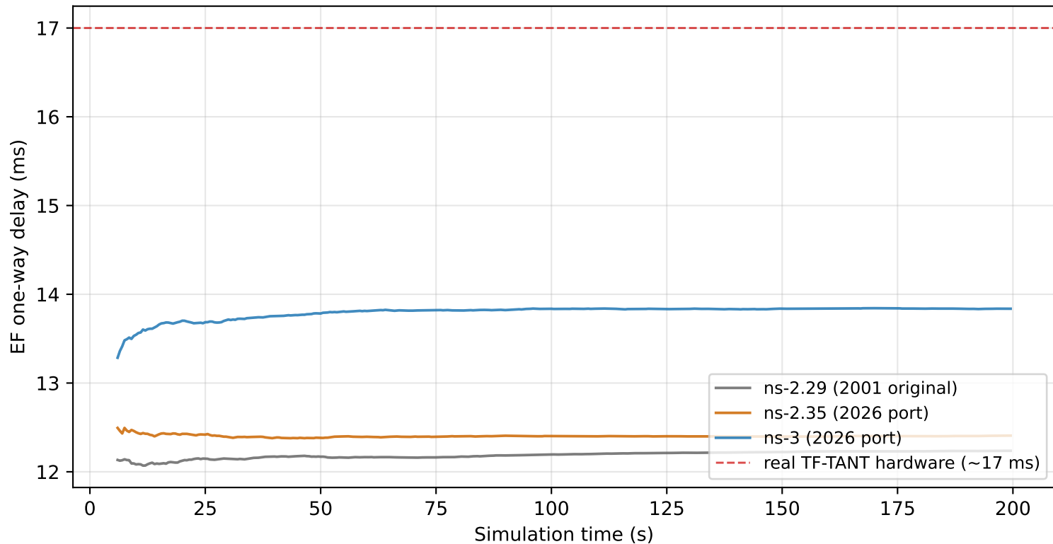
Scenario 1 — EF OWD at PQ scheduler, 512 B packets
