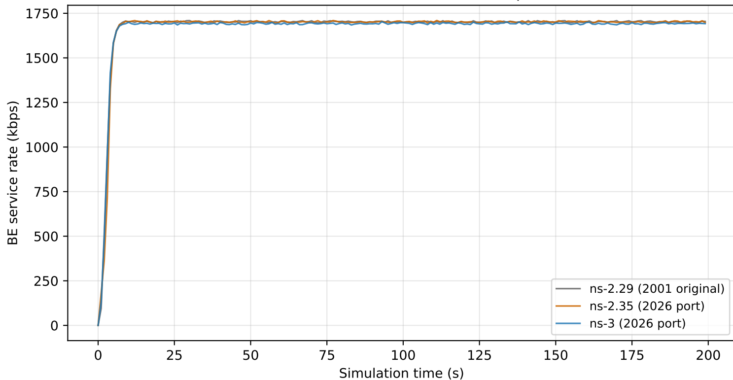
Scenario 1 — BE service rate, 512 B packets
