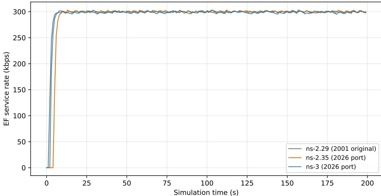
Scenario 1 — EF service rate, 512 B packets
