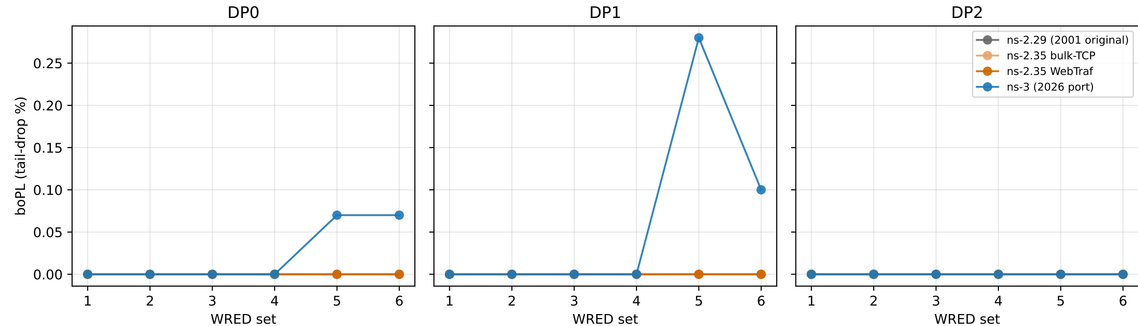
Scenario 2 — boPl (tail-drop %) per drop-precedence, 4-way comparison
