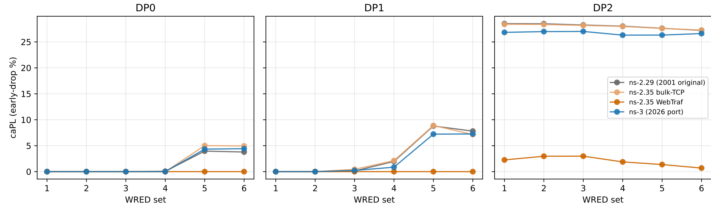
Scenario 2 — caPl (early-drop %) per drop-precedence, 4-way comparison
