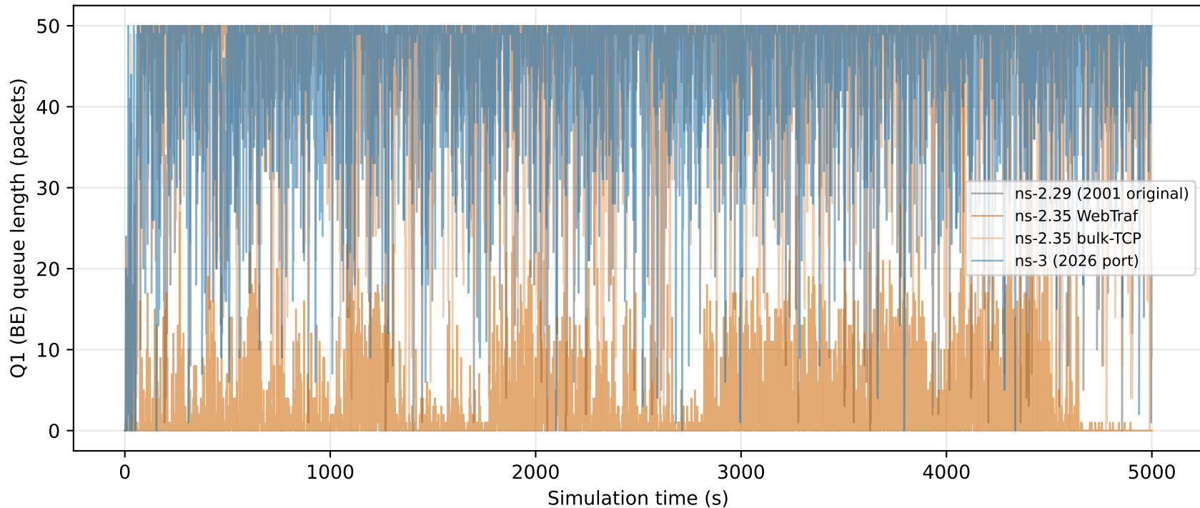
Scenario 2 — Q1 (BE) queue length, WRED set 1
