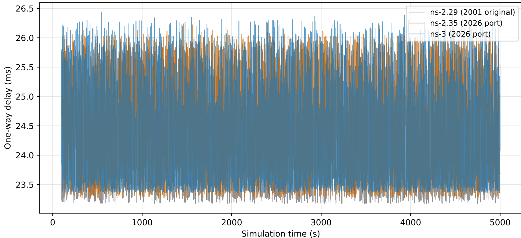
Scenario 3 — one-way delay (ms) (fullscale, warm-up t<100 skipped)
