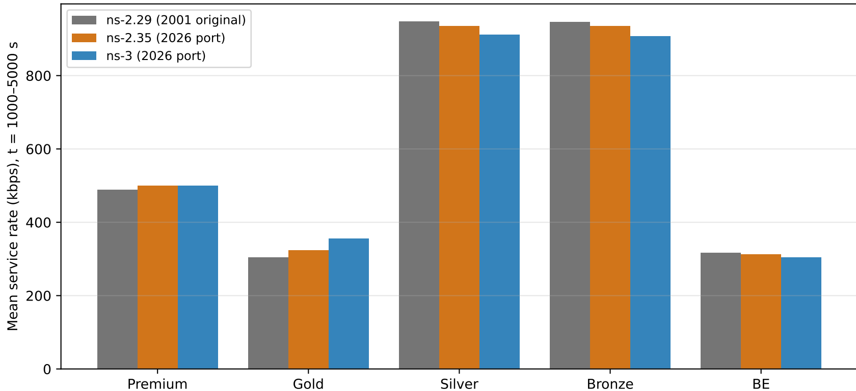
Scenario 3 — per-class service rates (three-way)
