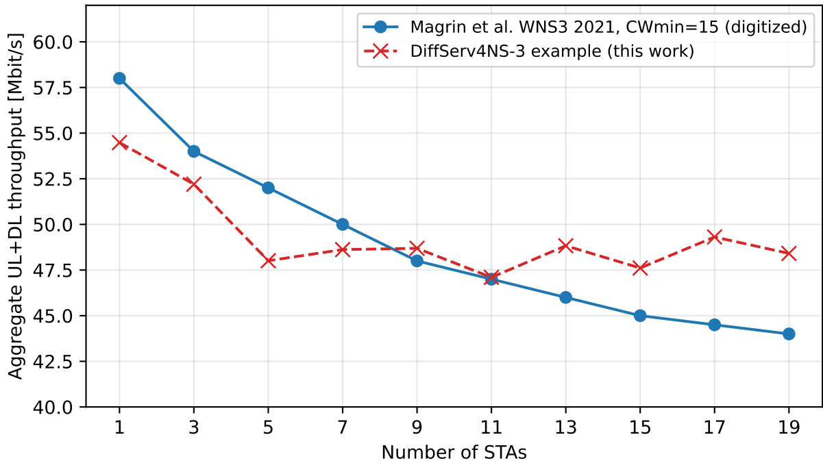
802.11ax SU saturation — MCS 5, 20 MHz, 5 GHz, BE
