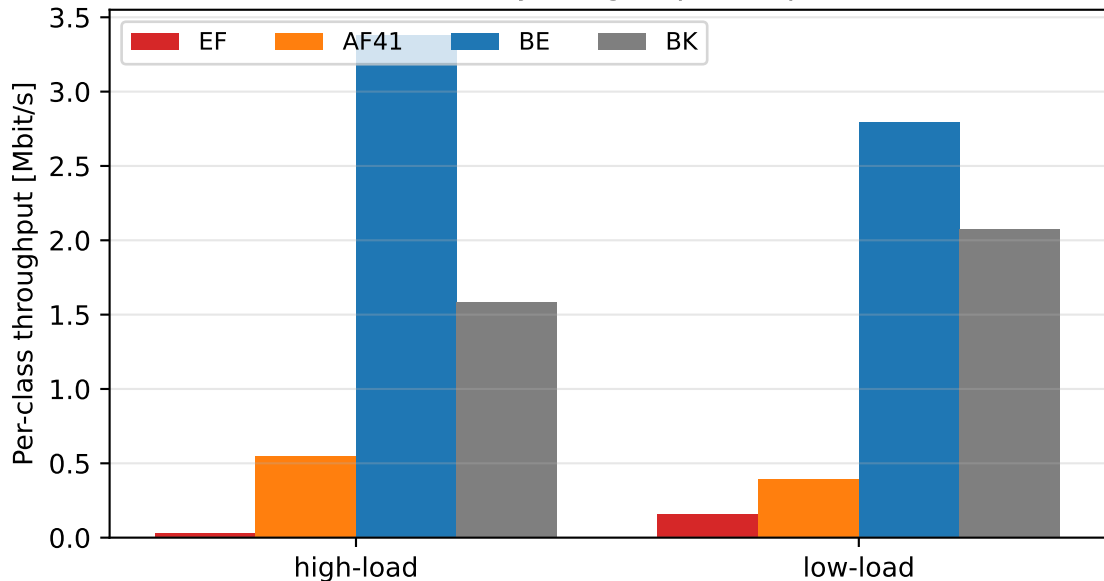
WMM mode = edca-only (single-queue qdisc, EDCA at L2)
