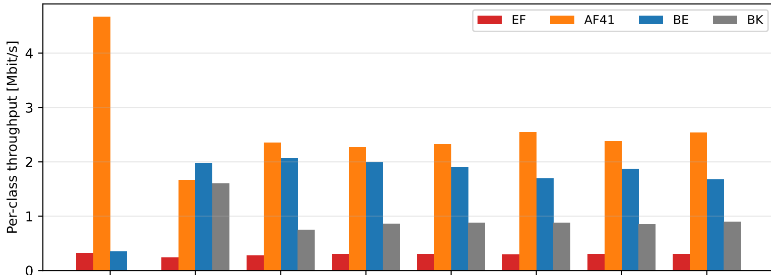
DiffServ4NS schedulers over 802.11a 6 Mb/s — saturating offered load, QoS off
