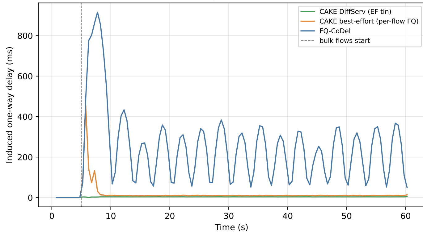
(a) Latency over time (ns-3)
