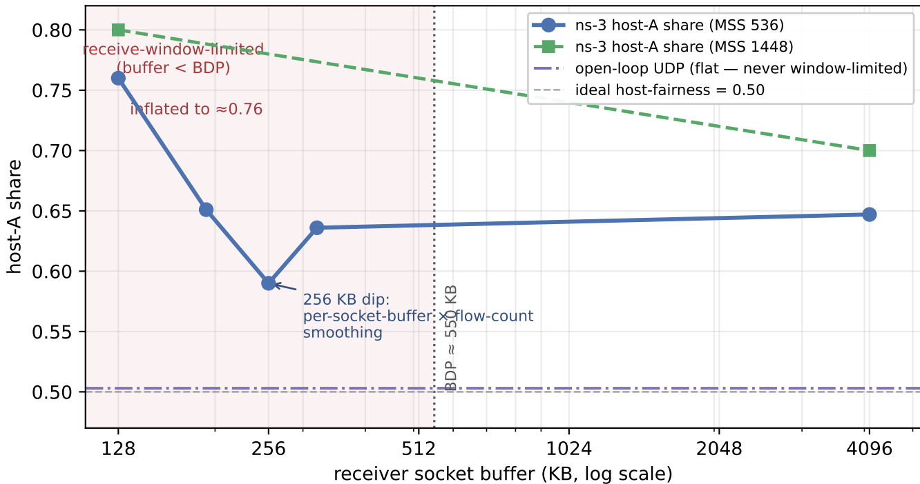
Socket-buffer window-limit leg (~11 pp) (4,1) split-destination, 100 Mbit/s, CAKE diffserv4 triple-isolate
