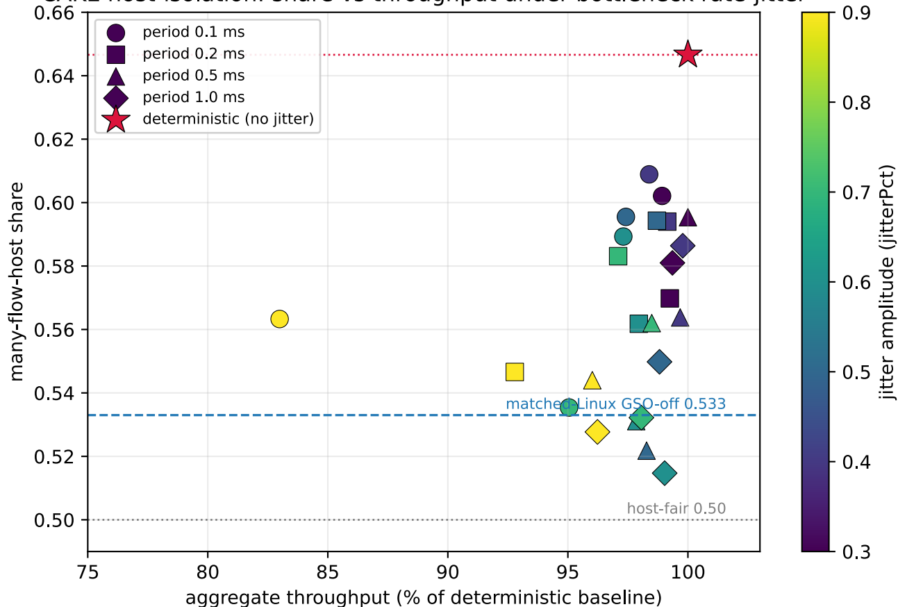
CAKE host-isolation: share vs throughput under bottleneck rate-jitter
