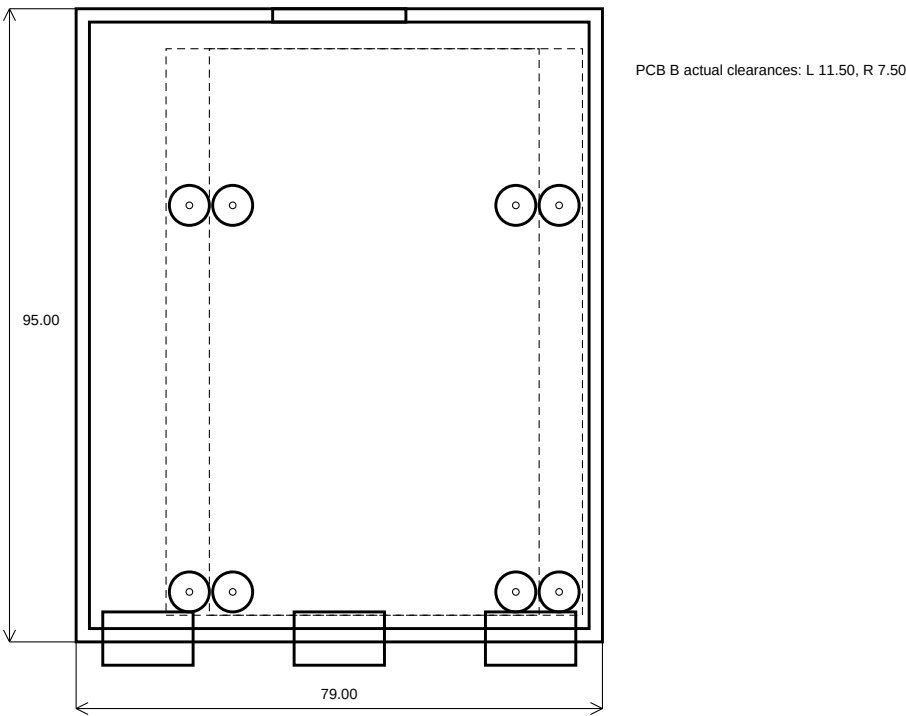
LOWER BASE - TOP
