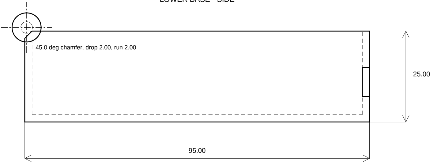
LOWER BASE - SIDE
