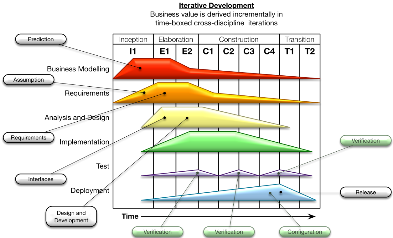
Figure 9.2: Development lifecycle
