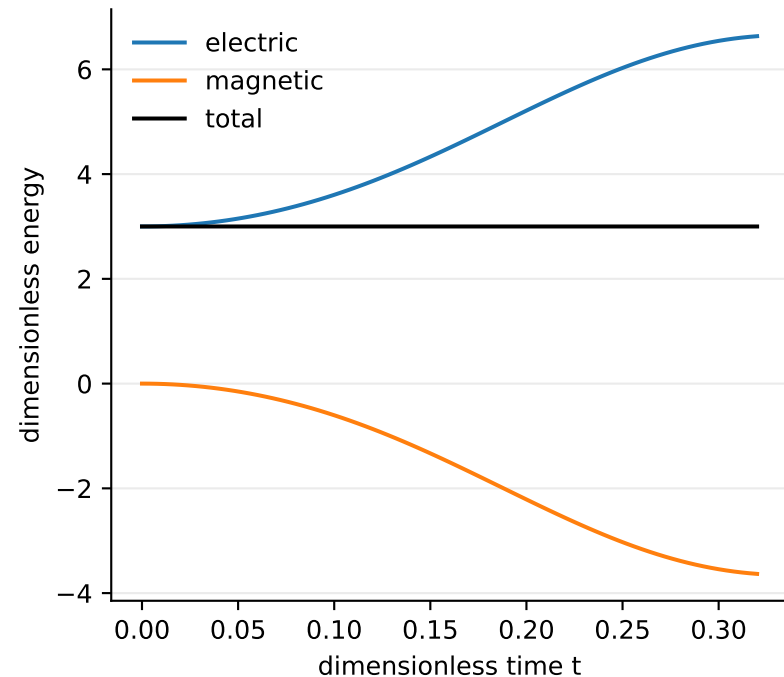
Exact Hamiltonian evolution
