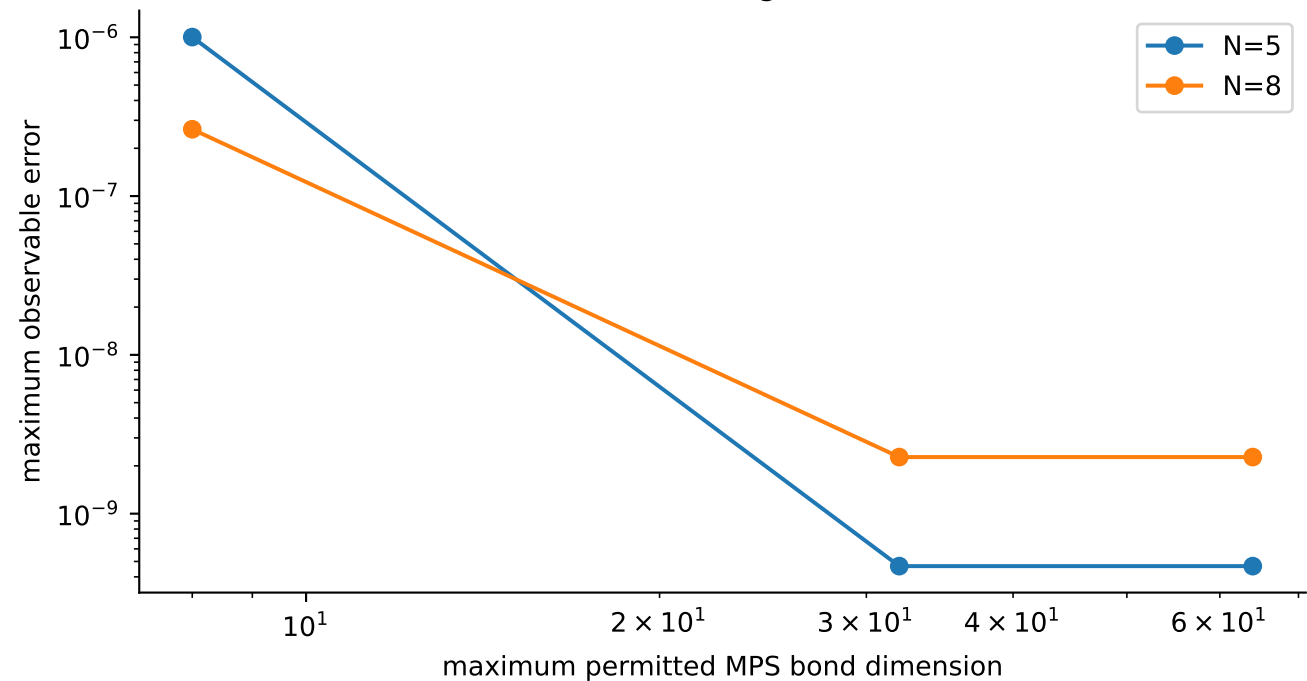
Direct MPS validation against ideal Trotter
