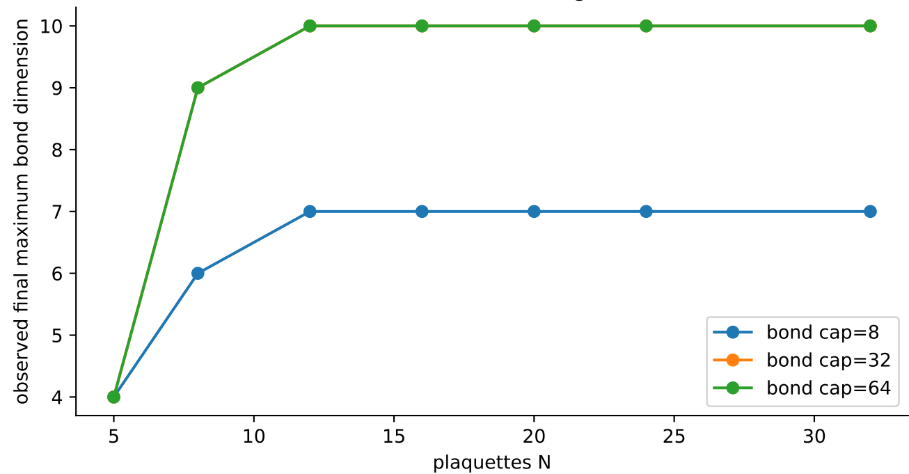
Direct-observable MPS scaling, t=0.32 , r=2
