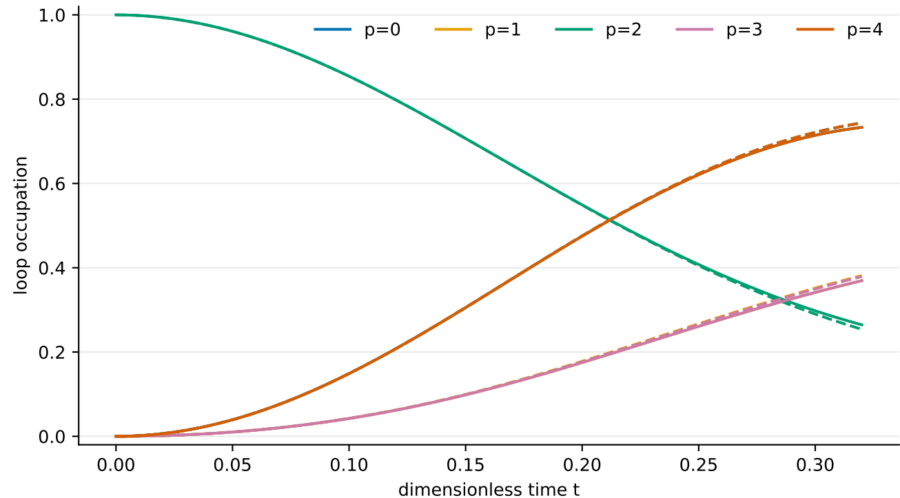
Five-plaquette occupations: exact (solid), Strang r=2 (dashed)
