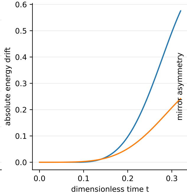
Term-ordering comparison at Strang r=2
