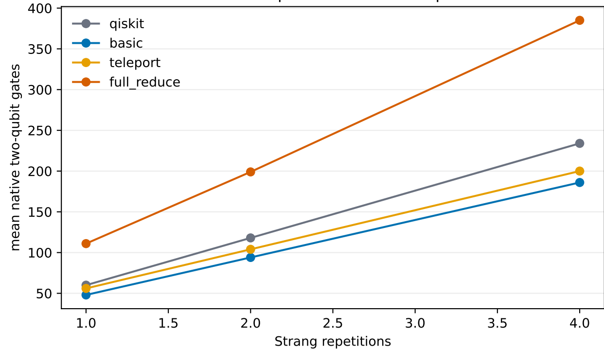
Generic five-qubit linear-ECR compilation
