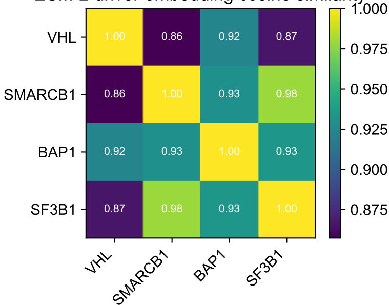
ESM-2 driver embedding cosine similarity
