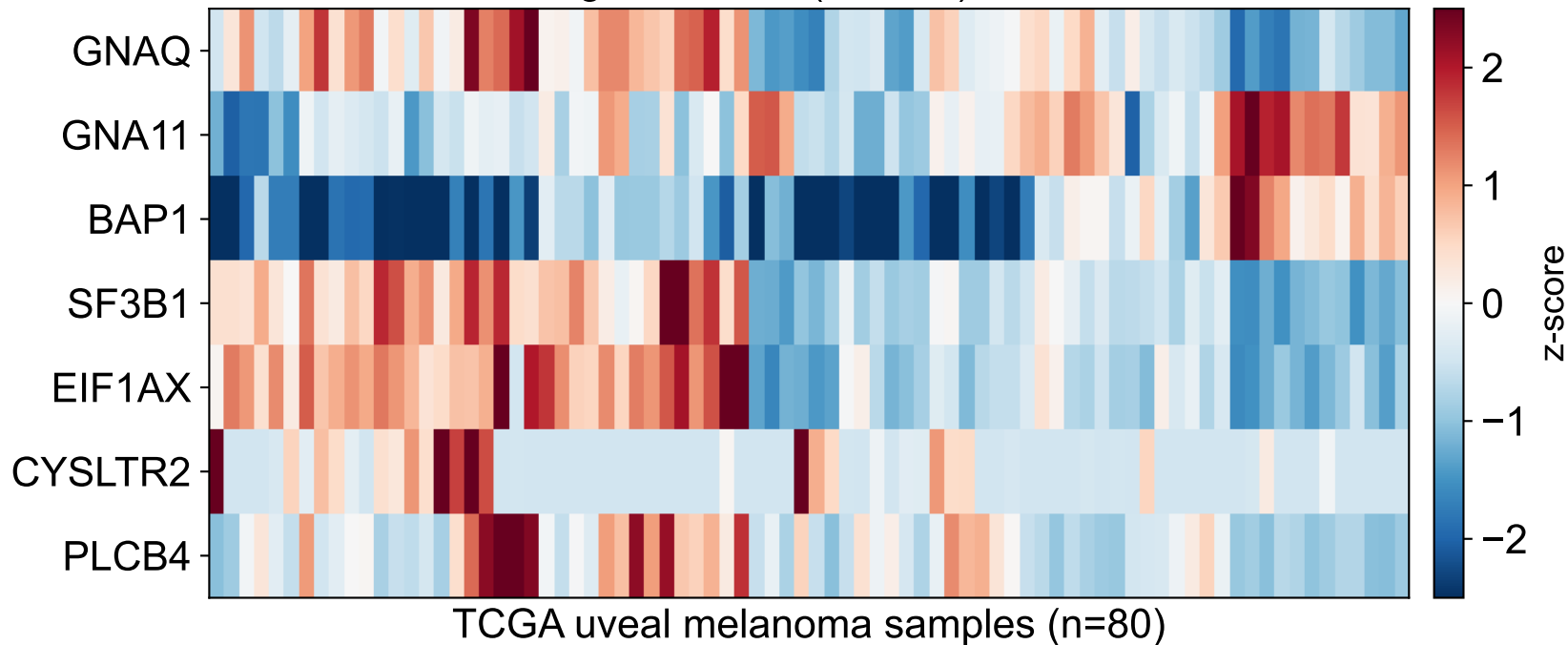
Driver gene mRNA (z-score), clustered
