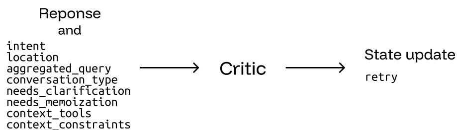
Figure 9 - Critic design, interfaces
