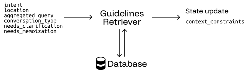
Figure 7 - Guidelines retriever, interfaces
