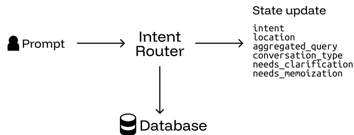
Figure 3 - Intent router, interfaces
