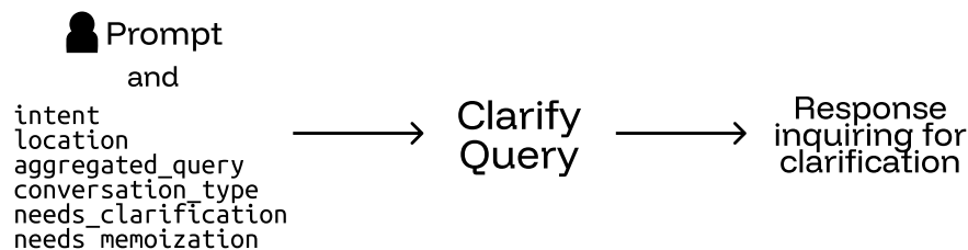
Figure 4 - Clarify query, interfaces
