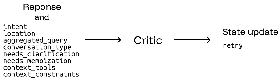
Figure 8 - Critic design, interfaces
