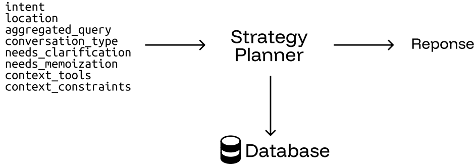
Figure 7 - Strategy planner, interfaces
