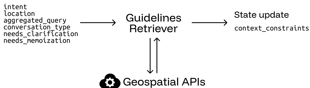
Figure 6 - Guidelines retriever, interfaces
