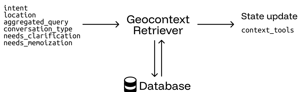
Figure 5 - Geocontext retriever, interfaces
