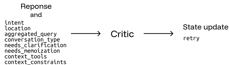
Figure 9 - Critic design, interfaces
