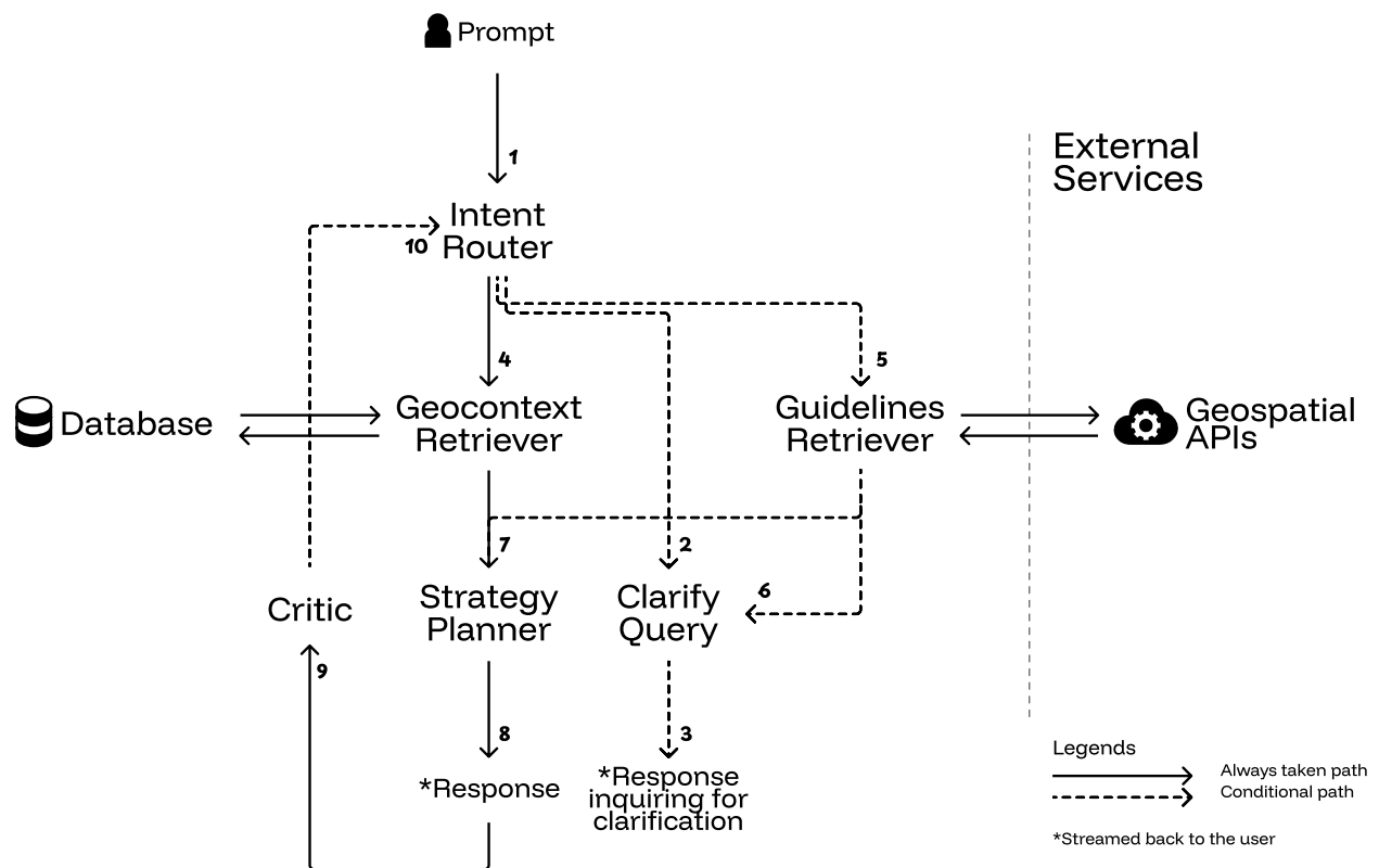
Figure 4 - AI agent architecture
