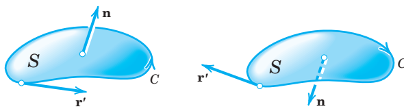
Fig. 254. Stokes's theorem
