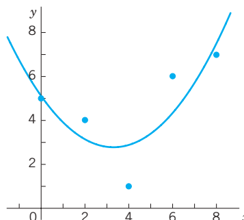
Fig. 448. Least squares parabola in Example 2
