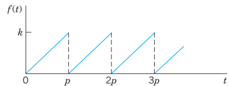
Fig. 139. Saw-tooth wave
