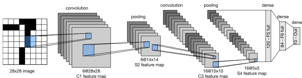
Figure : Architecture of LeNet-5 [6]
