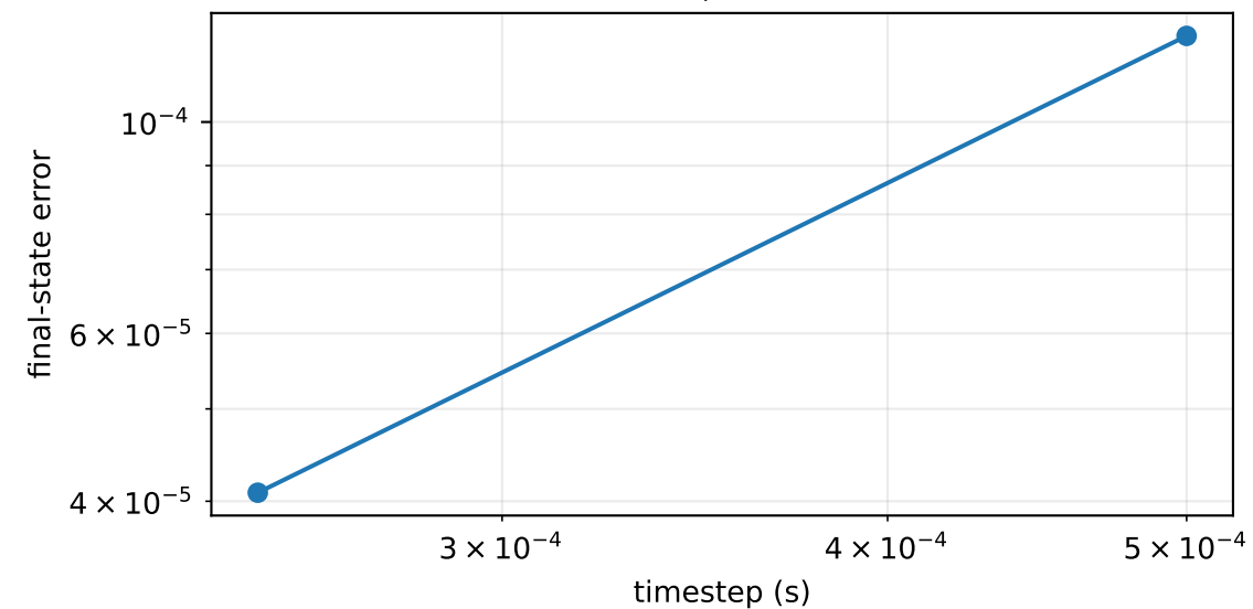
implicit BFGS / SVK / closed_form
