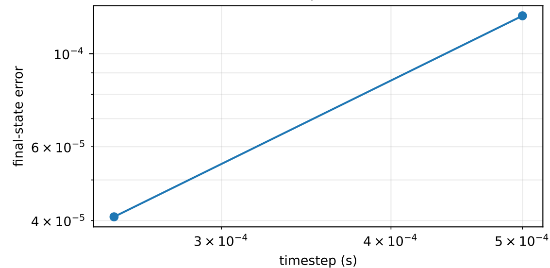
implicit BFGS / SVK / tangent_action
