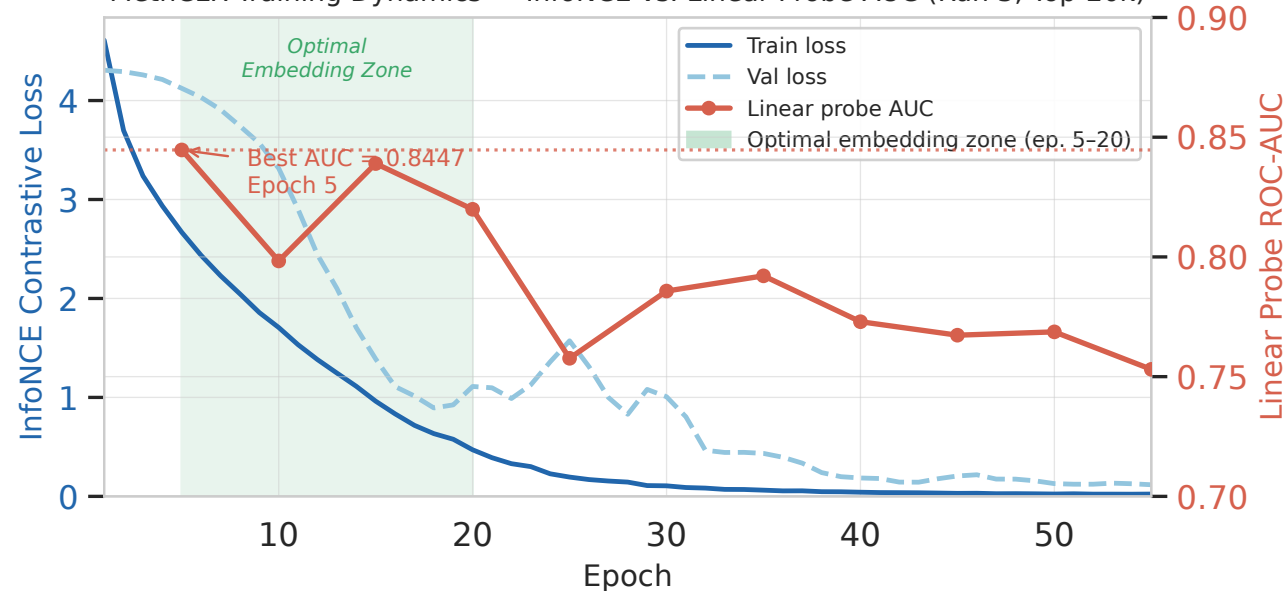
MethCLR Training Dynamics — InfoNCE vs. Linear Probe AUC (Run 3, Top-20k)
