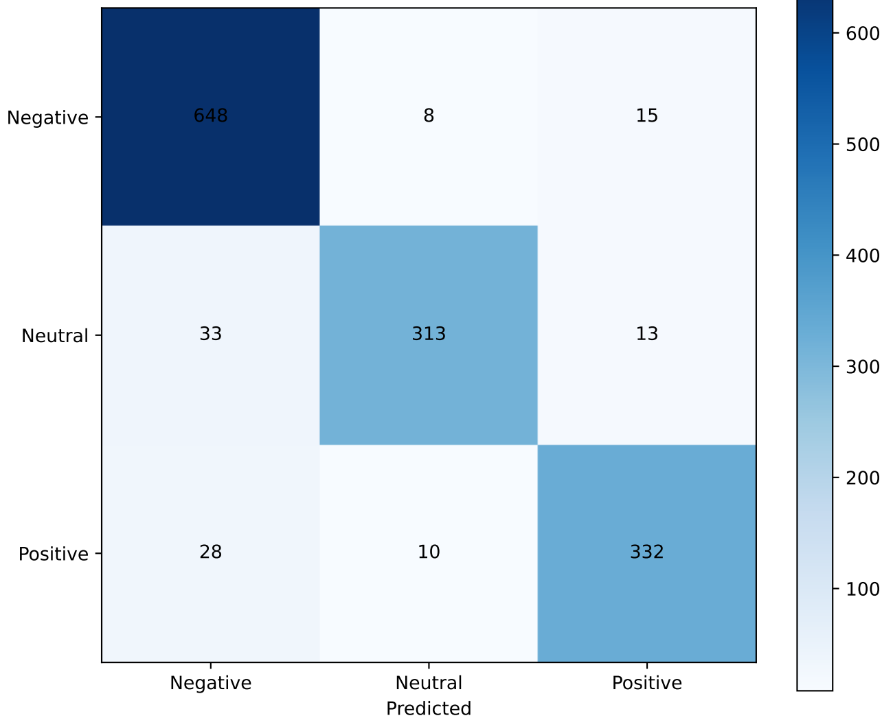
Confusion Matrix
