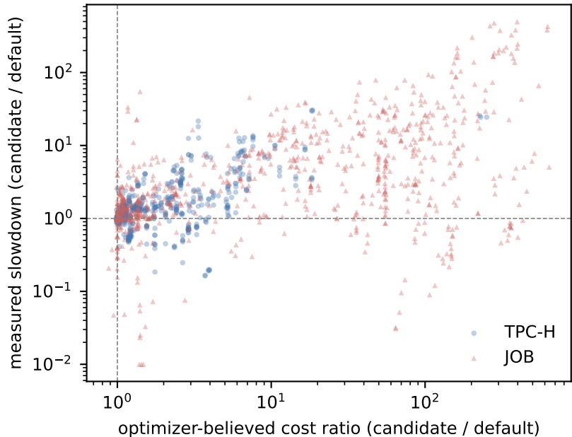
Optimizer belief vs. measured reality
