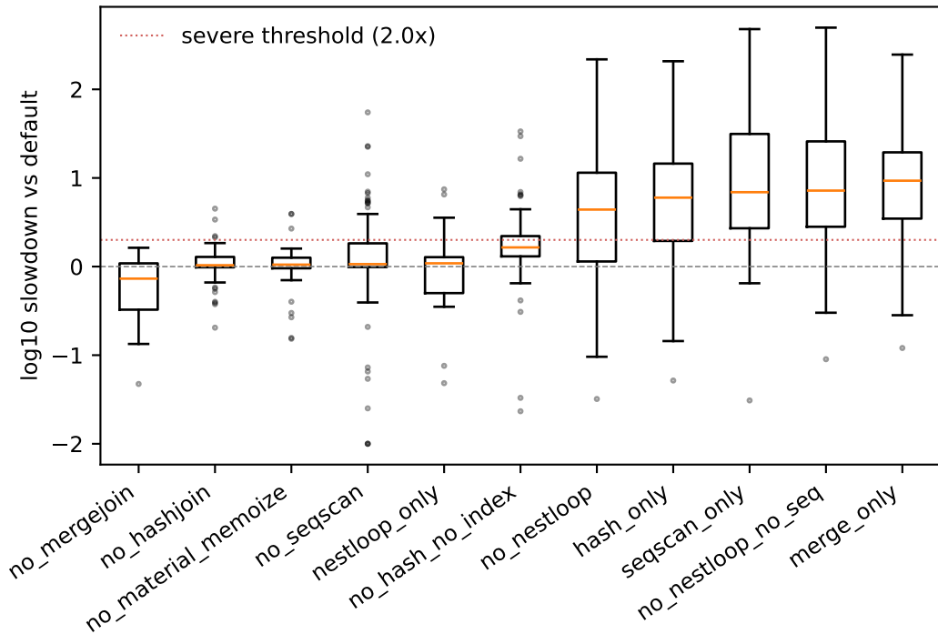
JOB: slowdown distribution by hint set
