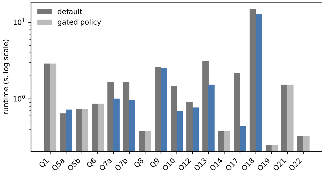
TPC-H certified live run: 9/17 steered, 0 severe, +15.0% net (Step 7i)
