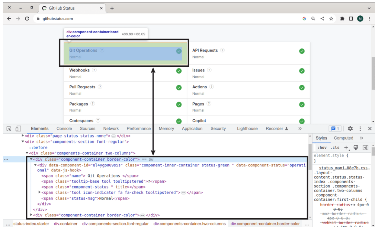
Figure 17.2 GitHub Status
