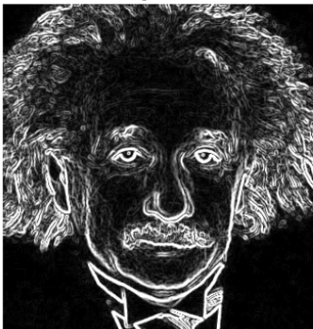
Using filter2D
