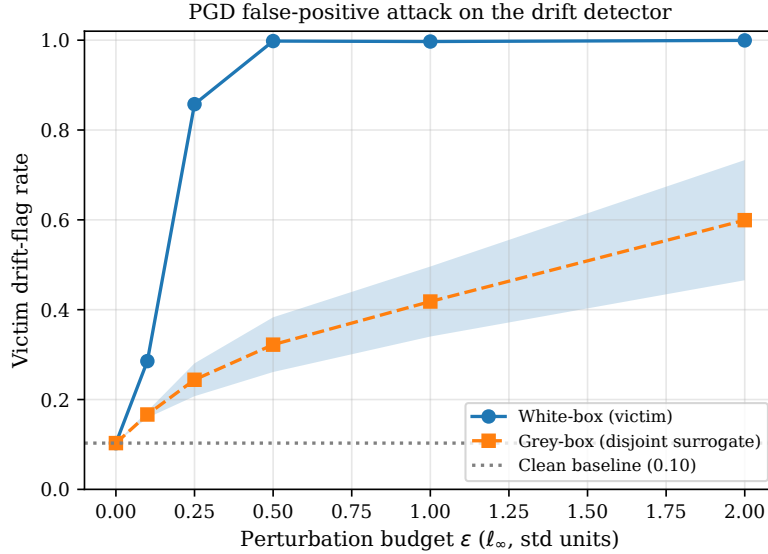
Figure 6.1: PGD false-positive attack on per-sample detection: fraction of perturbed known-class flows the victim flags as drifted versus the L_\infty budget, white-box against the victim and grey-box via surrogate transfer.
