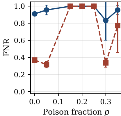
(c) FNR on PortScan
