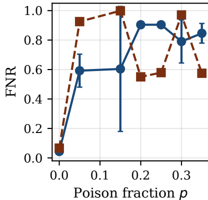
(b) FNR on DoS
