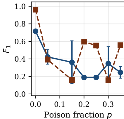
(a) Binary F1 (ATTACK)
