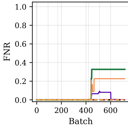
(c) FNR on DDoS
